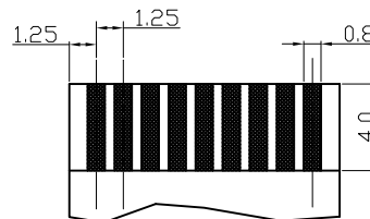
FFC/FPC DIMENSION THICKNESS 0.3±0.05mm
