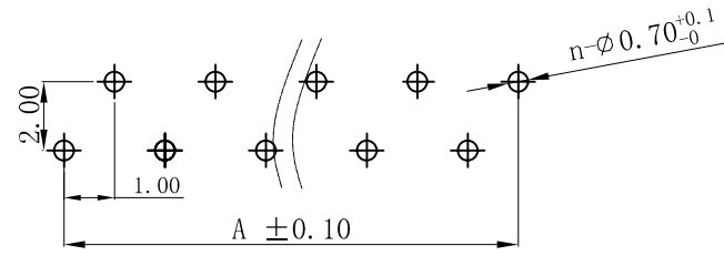
PCB Layout
